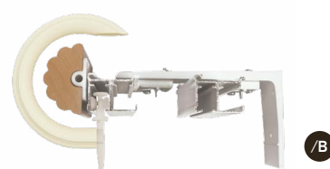
DOUBLE TRACK SYSTEM with "C" Rings, Cord Draw, Pinch Pleat, Fluted or Smooth, 1 3/8" or 2" D
